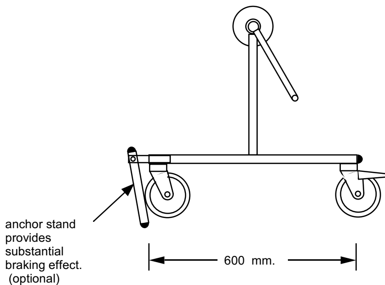
END VIEW
